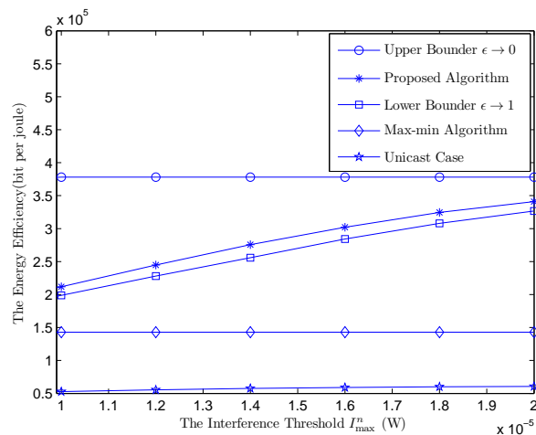
Fig. 4. The energy efficiency vs. the interference threshold I_{\max}^n .
