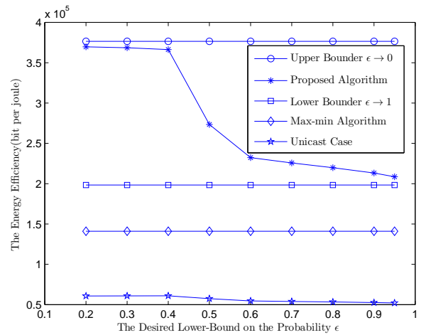
Fig. 2. The energy efficiency vs. the desired lower-bound on the probability \varepsilon .
