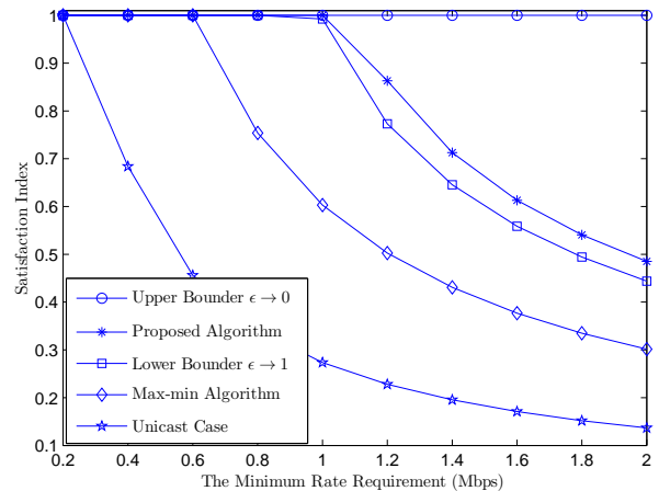
Fig. 9. The satisfaction index vs. the minimum rate requirement.
