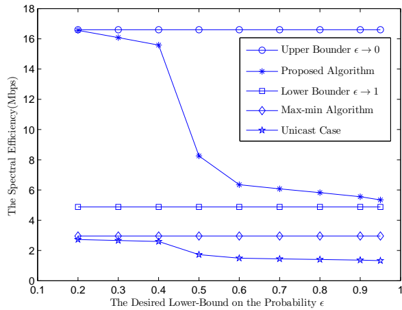
Fig. 3. The spectral efficiency vs. the desired lower-bound on the probability \epsilon .
