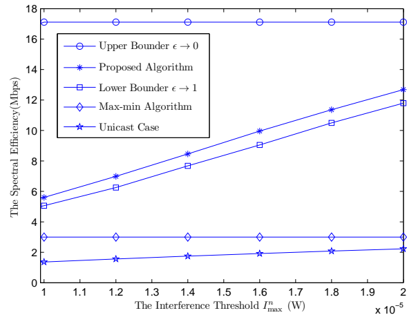
Fig. 5. The spectral efficiency vs. the interference threshold I_{\max}^n .
