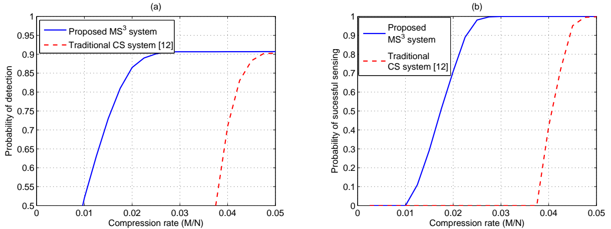
Fig. 6. Comparison between MS 3 and CS-based system [12]: (a) the probability of detection when the probability of false alarm is set to 10%, and (b) the probability of successful sensing which is defined as the probability of achieving both P_d \geq 90\% and P_f \leq 10\% . In simulations, the average SNR as received at CRs is 10 dB and the number of CRs is v = 22 .
