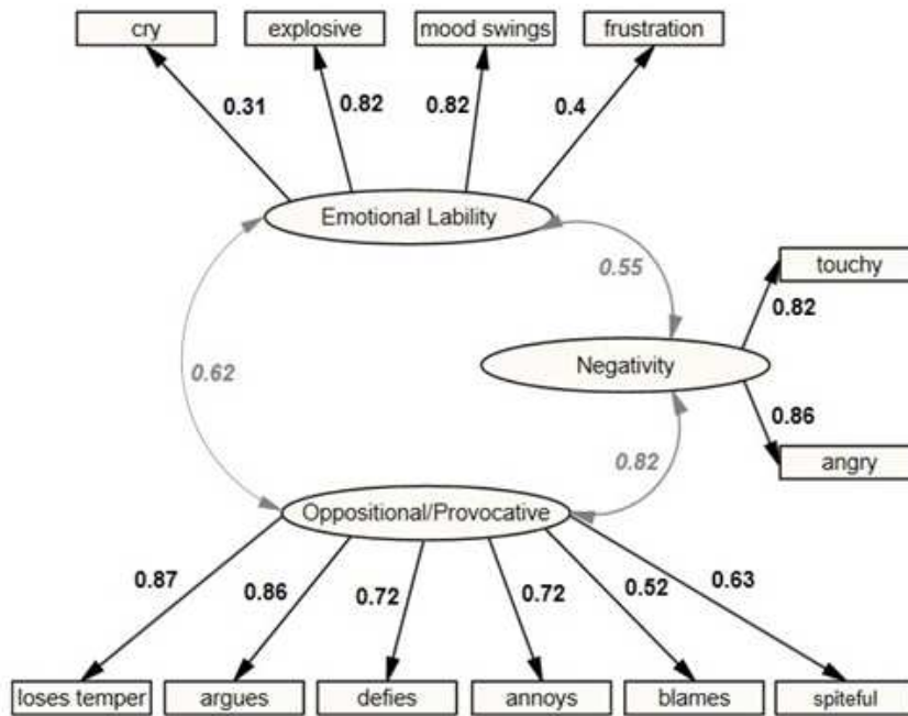
Figure 1(A) Screeplot of Exploratory Factor Analysis on the first split half ‘learning’ sample. (B) Path diagram of the CFA 3-factor Model (Model 8) derived from the second split-half ‘testing’ sample. Rectangles represent observed items and ellipses represent the latent variables (factors). The parameters printed by the black straight arrows represent the standardized loadings and the coefficients on the curved grey arrows represent the correlations between factors ( p < 0.05 in all cases).
