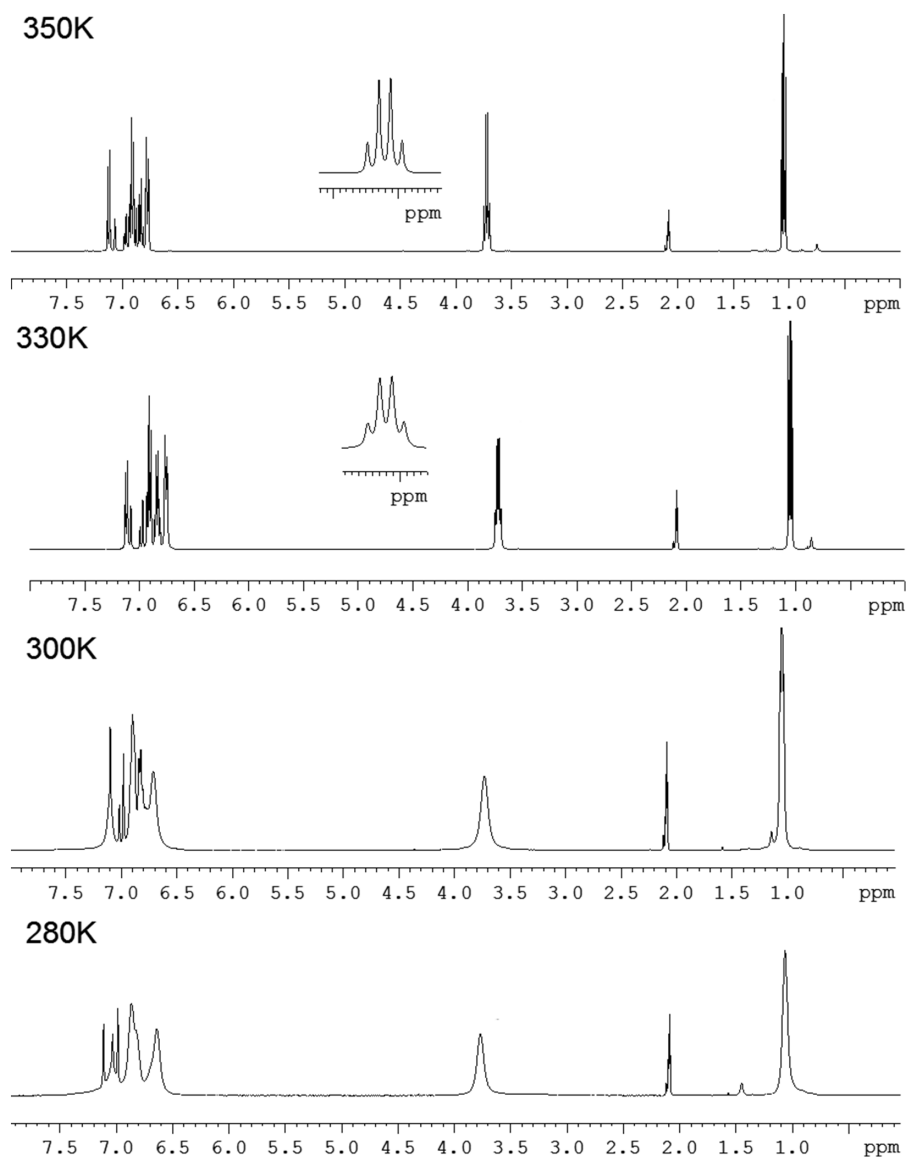
Figure 7 | Variable temperature 1 H NMR spectra of bis-amide ligand 7b (400 MHz, d 8 -toluene), confirming slow conformational change at room temperature.
