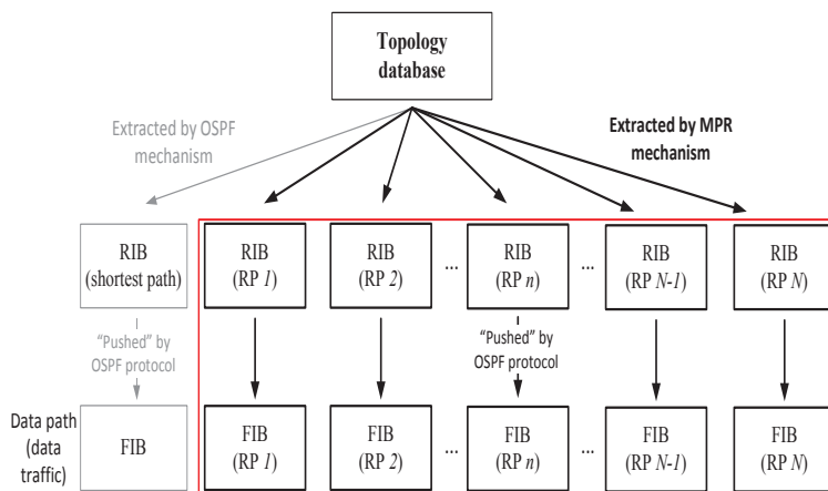
Figure 1: Data flow under conventional routing (left-hand side, thin grey lines) and under MP routing (thick black lines).
