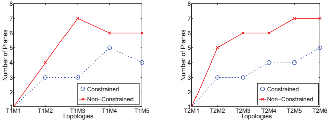
(a) Number of planes for the 1st set of topologies
