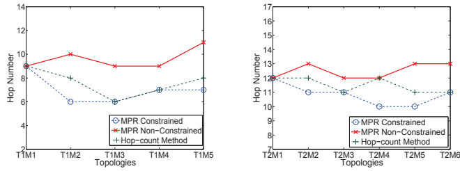
(a) The maximum hop number for the 1st set of topologies
