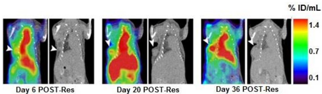
Suppl. Fig. 5. Progressive increase in uptake of [^{18}\text{F}] AH113804 at the tumor site post tumor resection. PET and CT image of a same tumor bearing mouse acquired on Day 6, Day 20 and Day 36 post resection showing uptake of [^{18}\text{F}] AH113804 at 60 min p.i. The recurrent tumour is clearly visible on the right flank of the animal (white arrowhead).
