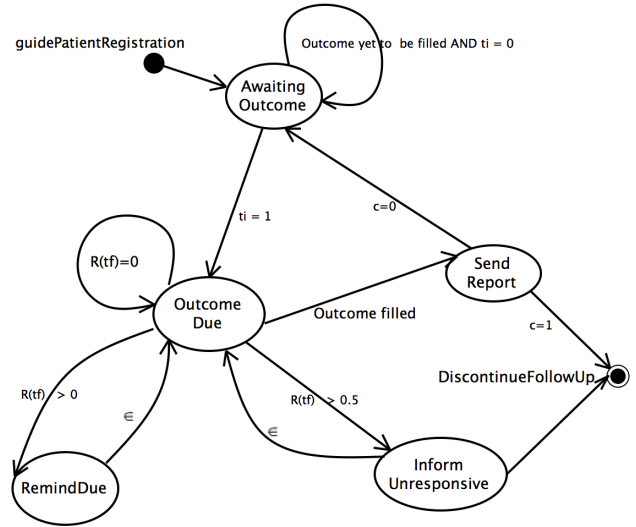
Figure 2: The PatientFollowUp agent Finite State Machine
