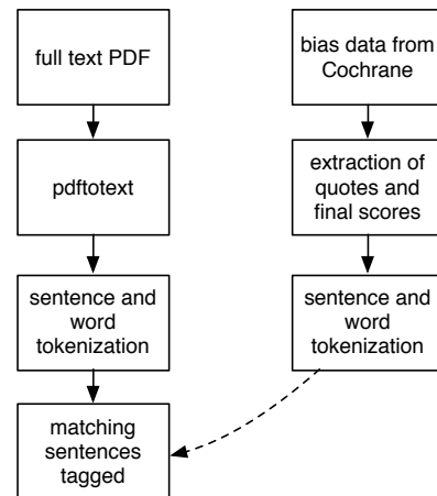
Figure 3: Corpus construction processing
