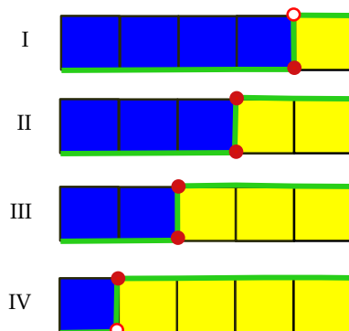
Figure 4. Phases of the \mathfrak{su}(5) theory with fundamental representation 5 matter. The blue/yellow boxes correspond to decorating with \pm . The green lines and red dots will play a role later on in understanding the flops between these phases: red dots correspond to extremal points that can be flopped, whereas white dots correspond to flops that would map out of the \mathfrak{su}(5) phases to the \mathfrak{u}(5) phases.
