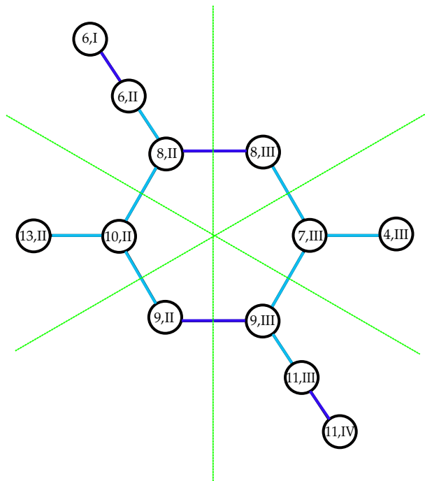
Figure 11. The phase diagram for SU(5) with fundamental and anti-symmetric matter, as derived from flops among the decorated box graphs/anti-Dyck paths in figure 9. Identification along the dark blue lines yields the phase diagram of the anti-symmetric representation, identification of nodes along the light blue lines yields the phase diagram, which is a line, for the fundamental representation. The curious observation which is drawn in terms of the green dotted lines is, that this diagram can be cut up into pairs of Dynkin diagrams of E_6 , D_6 and A_6 , respectively. The case of the E_6 flop diagram (corresponding to cutting the graph by the NE to SW diagonal) is discussed later in terms of the E_6 codimension-three fibers in section 8.4.
