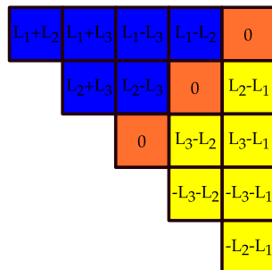
Figure 22. The box graph of the \mathrm{Sp}(3) theory with \Lambda^2 \mathbf{6} . Blue boxes indicate the sign of the corresponding weight is plus, yellow indicates negative, and orange that there is no way to associate a definite sign.
