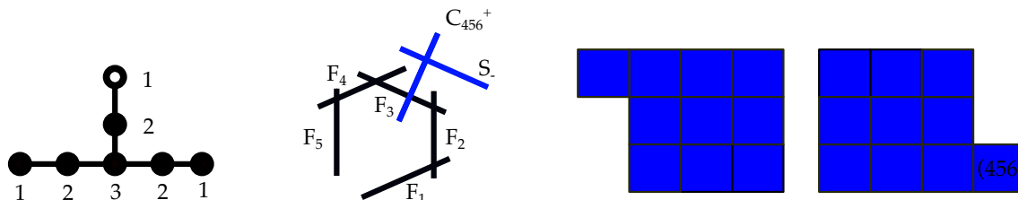
Figure 29. Example phase and fiber type of the U(6) theory with \Lambda^3 \mathbf{6} , corresponding to trivial monodromy action, with standard Kodaira IV^* fiber. Description of the various diagrams is as in figure 28.
