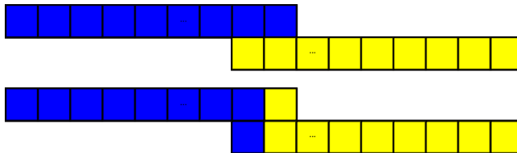
Figure 38. The phases of the \text{SO}(2n) theory. Blue indicates the box is decorated with a plus sign and yellow with a negative.
