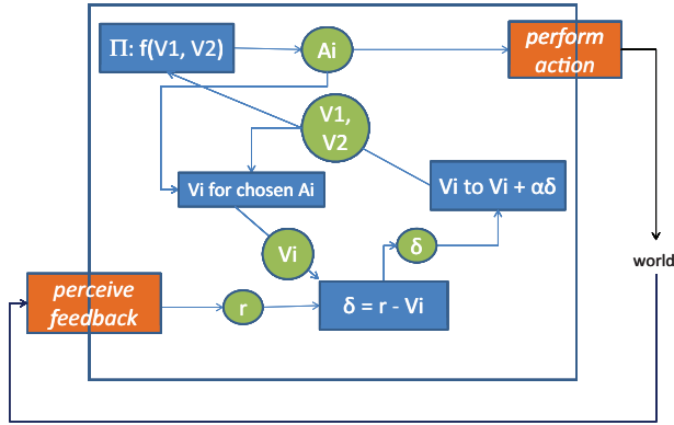
Figure 1. Simplified Actor-Critic Model
