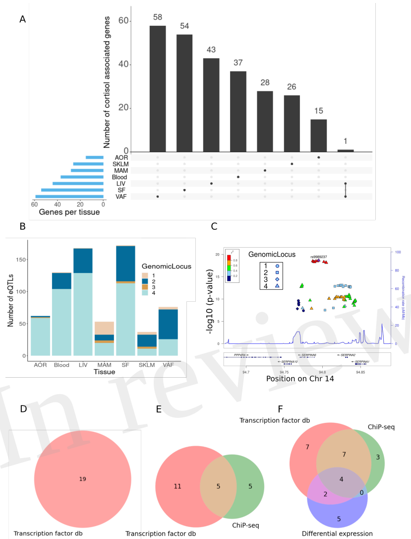
Figure 1: Identification of cortisol-associated trans-genes across STARNET tissues (FDR = 15%). (A) Upset plot showing the distribution of trans-genes across STARNET tissues, including genes shared by multiple tissues. Tissues include atherosclerotic aortic root (AOR), skeletal muscle (SKLM), internal mammary artery (MAM), blood (Blood), liver (LIV), subcutaneous fat (SF) and visceral abdominal fat (VAF). (B) Distribution of trans-eQTLs across tissues and coloured by genomic locus (LD block) of associated SNP. (C) LocusZoom plot 30 showing the location of cortisol associated SNPs within defined LD blocks. (D) Venn diagrams where groupings represent different sources used to identify GR-linked trans-genes in liver, (E) visceral abdominal fat and (F) subcutaneous fat. These sources include transcription factor databases (db), ChiP-seq from perturbation-based experiments 23 and differential expression of dexamethasone treated mice 24 .
