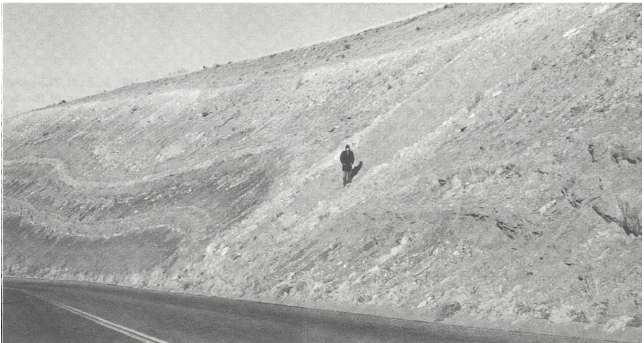
Figure 17. Oval collapse chimney in red Permian mudstones filled with Tertiary or younger fluvial sand and gravel. The collapse chimney filling is slightly cemented. Note the downwarping of the Permian enclosing beds. Figure on collapse chimney for scale. Photograph is of an area on Texas Highway 136 approximately 5 km (3 mi) north of Borger in Hutchinson County, Texas.
