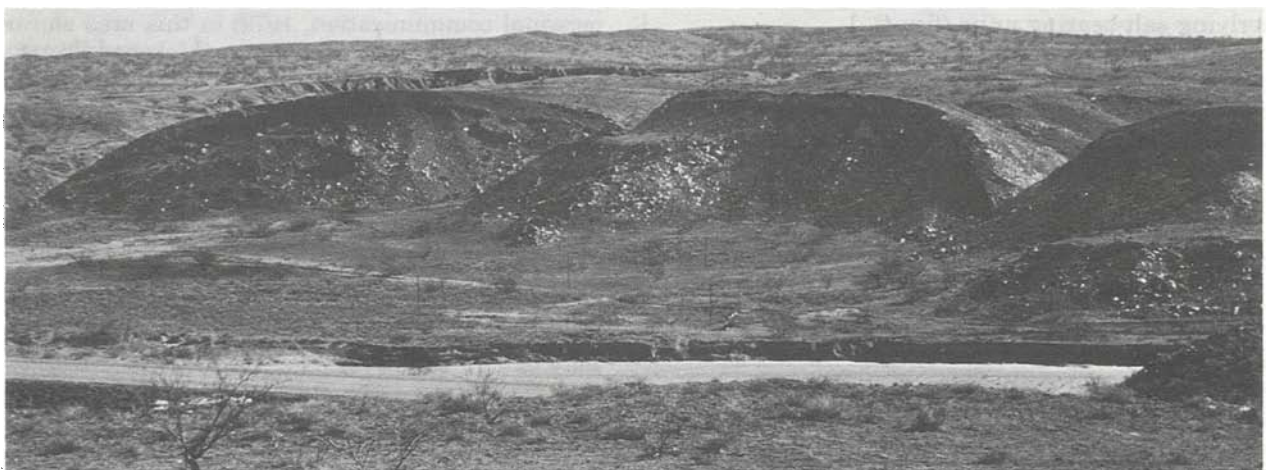
Figure 21. Folded red Permian mudstones capped by the Alibates Dolomite Lentil in the Canadian River Valley adjacent to Texas Highway 136 approximately 10 km (6 mi) north of Borger, Texas.
