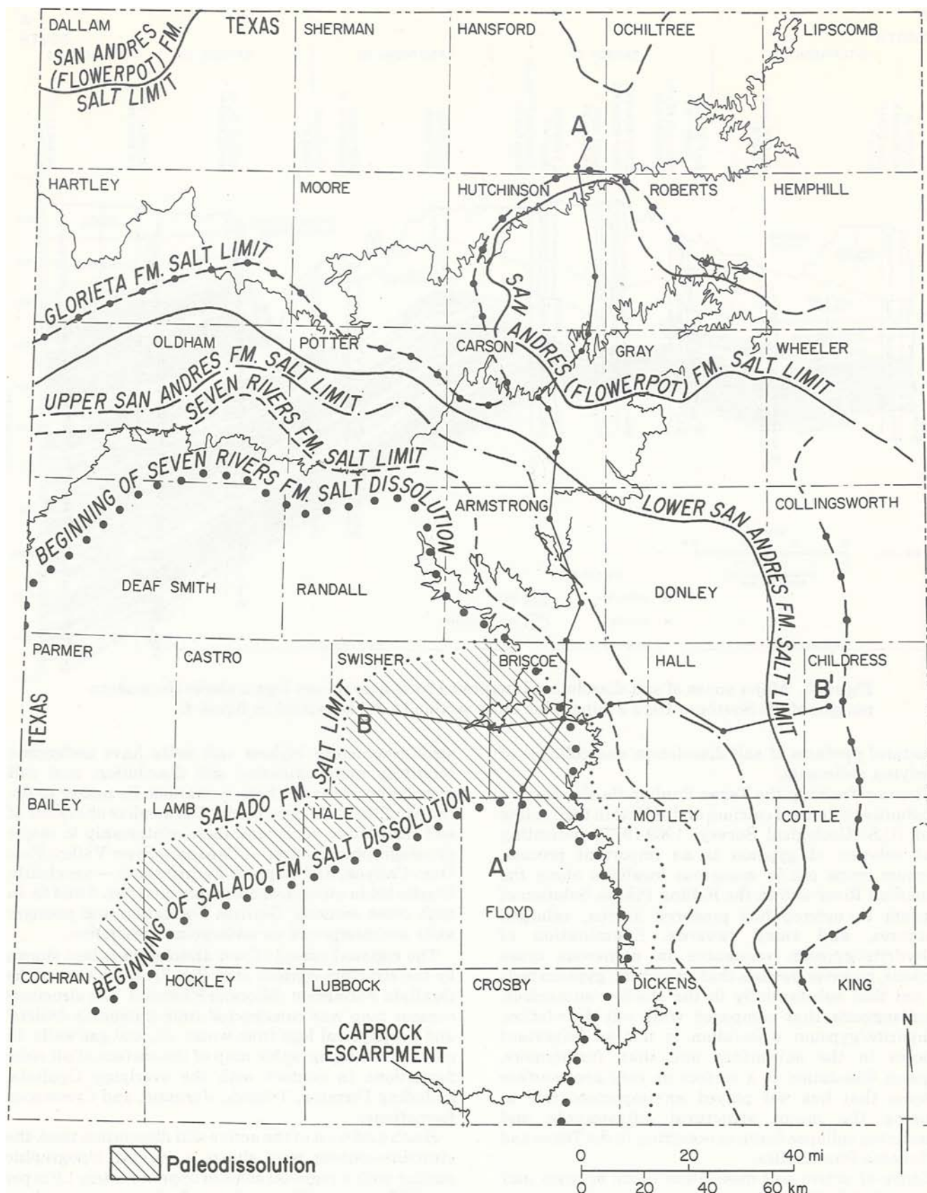
Figure 4. The zone of active salt dissolution occurs north and east of the beginning of salt dissolution lines and parallels the Caprock Escarpment. Small additional areas of salt are undergoing dissolution in northwest Dallam, northeast Hansford, and northwest Ochiltree Counties.
