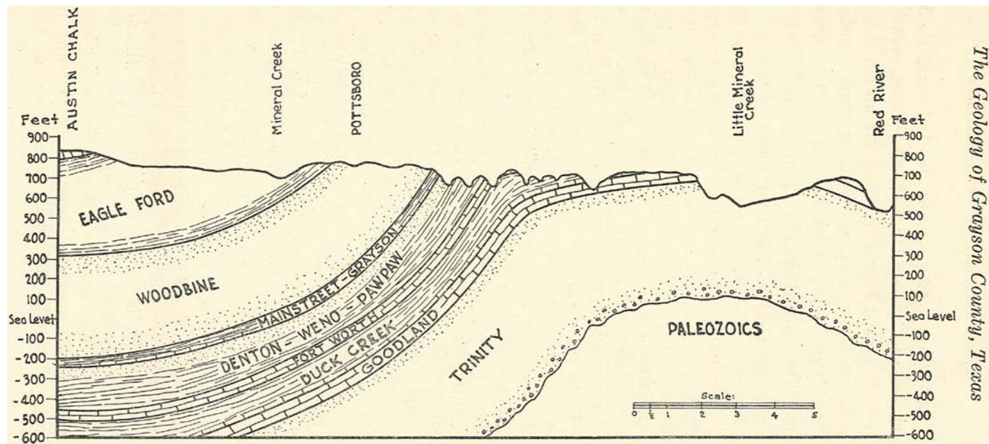
FIG. 2. Structure section across the Preston Anticline from a point on Red River, one mile northeast of Preston, southward through Pottsboro.
