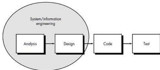
Gambar 1. Waterfall Model [6]
