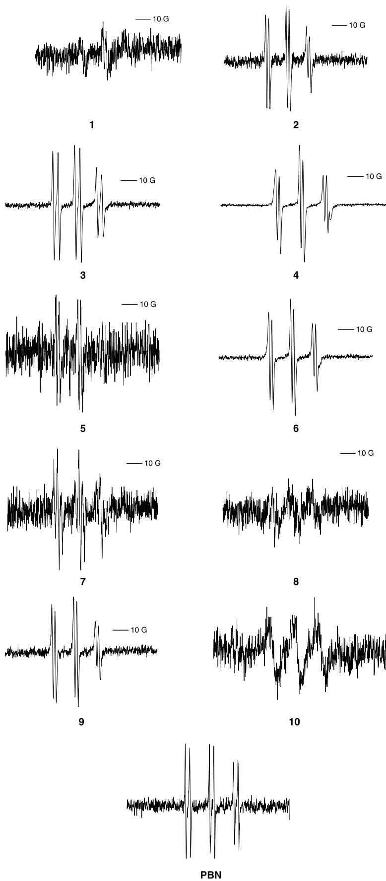
Figure 4. EPR spectra of nitrones 1-10 and PBN (10 mM) with \cdot\text{CH}_3 generated by Fenton's reaction ( \text{Fe}^{2+}/\text{H}_2\text{O}_2 :100/100 \mu\text{M} ) in \text{H}_2\text{O}/\text{DMSO}/\text{DMF} : 30/60/10 (v/v). Gain: 5.64 \times 10^4 .
