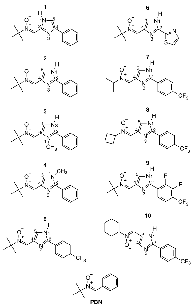
Figure 1. Structure of the imidazolyl nitrones: 1, ( Z ) α [4 phenyl 1 H imidazol 2 yl] N tert butyl nitronone; 2, ( Z ) α (2 phenyl 1 H imidazol 4 yl) N tert butyl nitronone; 3, ( Z ) α [1 methyl 2 phenyl 1 H imidazol 5 yl] N tert butyl nitronone; 4, ( Z ) α [3 methyl 2 phenyl 1 H imidazol 5 yl] N tert butyl nitronone; 5, ( Z ) α [2 (4 trifluoromethylphenyl) 1 H imidazol 4 yl] N tert butyl nitronone; 6, ( Z ) α [2 (2 thiazolyl) 1 H imidazol 4 yl] N tert butyl nitronone; 7, ( Z ) α [2 (4 trifluoromethylphenyl) 1 H imidazol 4 yl] N isopropyl nitronone; 8, ( Z ) α [2 (4 trifluoromethylphenyl) 1 H imidazol 4 yl] N cyclobutyl nitronone; 9, ( Z ) α [2 (2 fluoro 3 fluoro 4 trifluoromethylphenyl) 1 H imidazol 4 yl] N tert butyl nitronone; 10, ( Z ) α [2 (4 trifluoromethylphenyl) 1 H imidazol 4 yl] N cyclohexyl nitronone.
