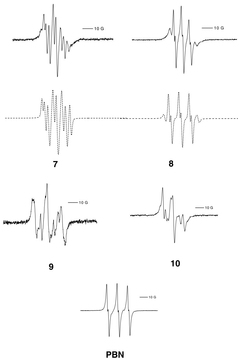
Figure 5. EPR spectra of nitrones 1–10 and PBN (10 mM) with \text{CH}_3 \cdot \text{CH} \cdot \text{CH}_3 prepared in benzene from isobutyric acid and lead tetraacetate (45/45 mM). Gain: 5.64 \times 10^3 . Solid lines: experimental spectra; dashed lines: simulated spectra.
