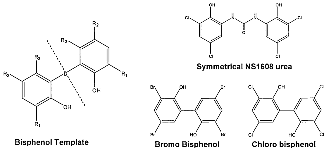
Figure 1.19: Symmetrical bisphenols
