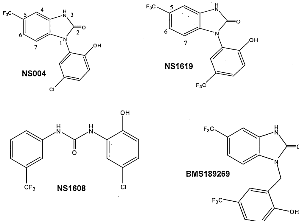
Figure 1.11: Benzimidazolone compounds
