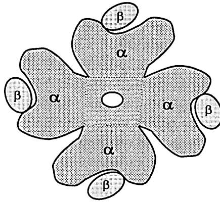
Figure 1.2: Topological structure of BK Ca channels
