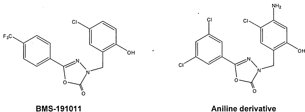
Figure 1.16: Oxadiazolones
