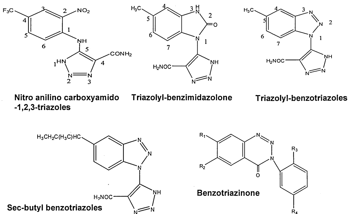
Figure 1.17: Triazoles I
