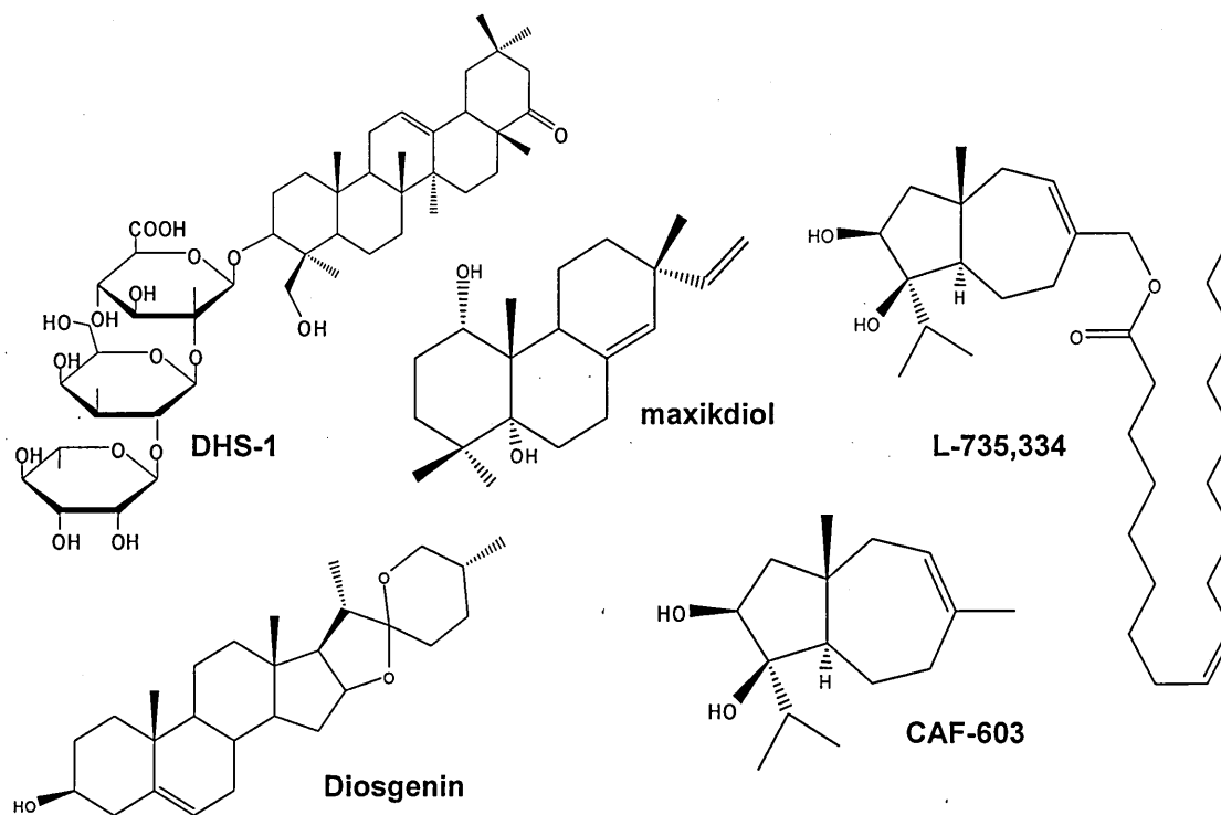
Figure 1.6: Terpinoids
