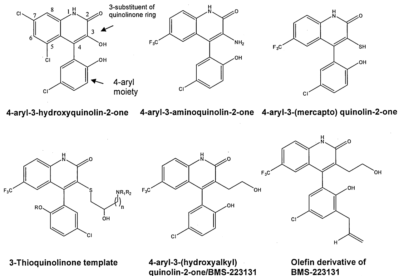
Figure 1.14: Substituted quinolin-2-ones
