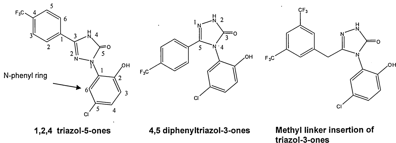
Figure 1.15: Triazolones
