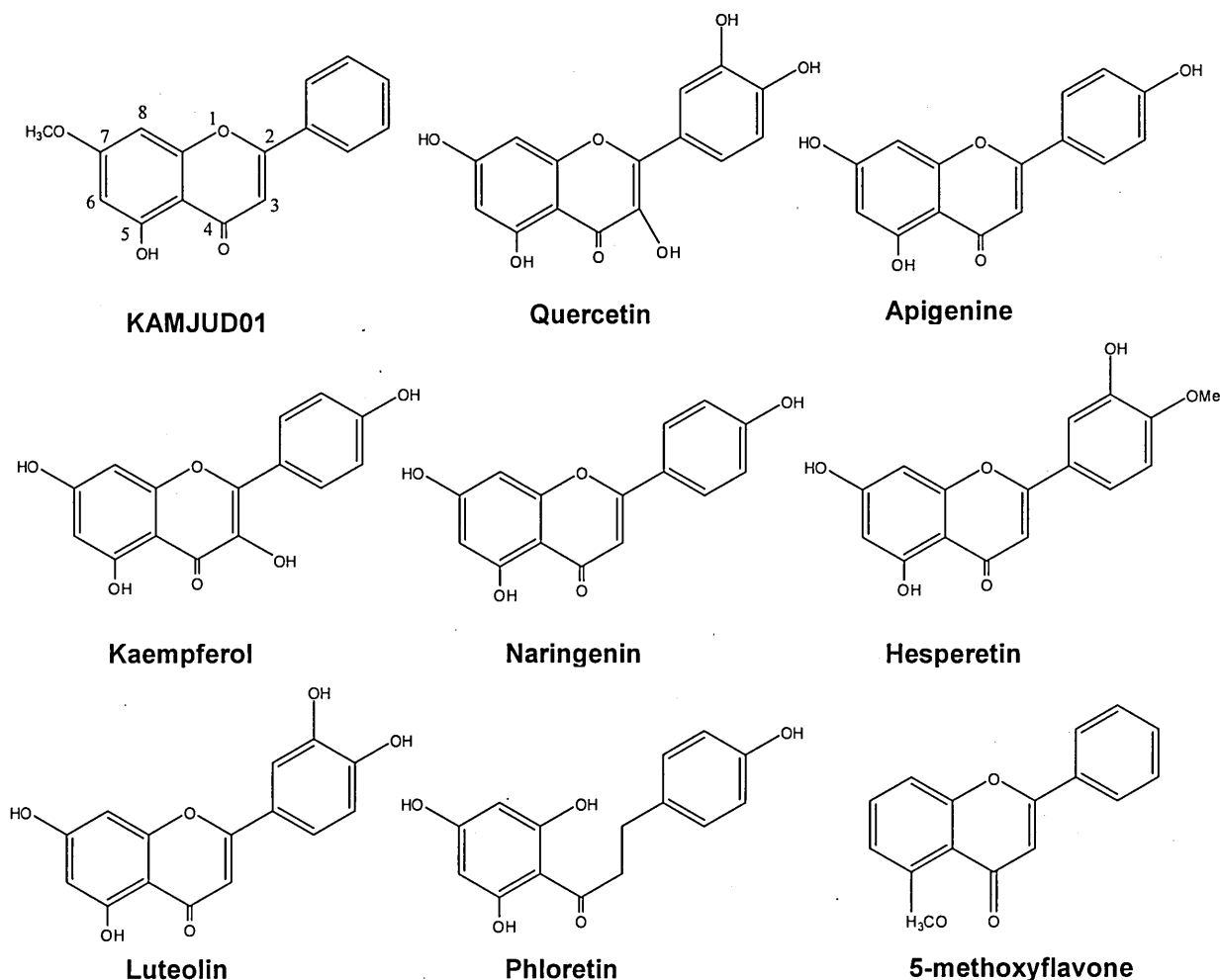
Figure 1.12: Flavonoids
