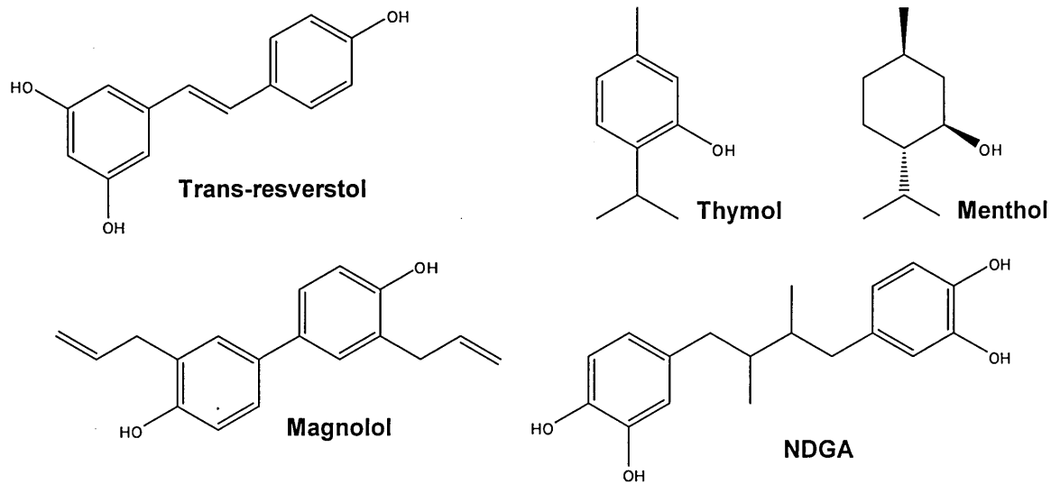
Figure 1.7: Phenolic compounds
