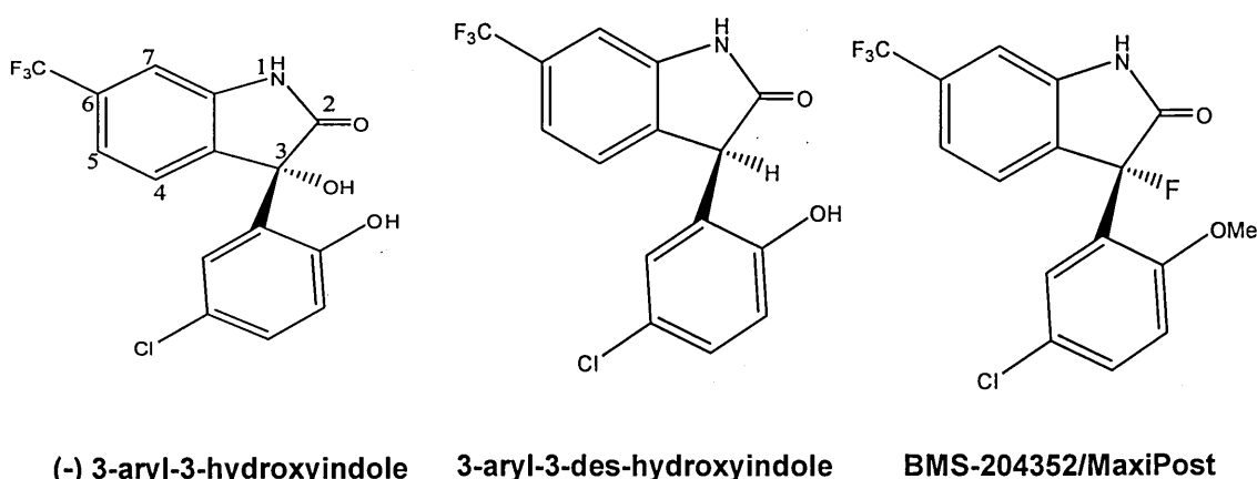
Figure 1.13: Oxindoles
